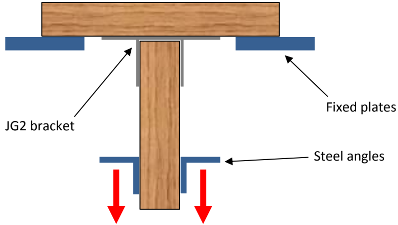
Figure 2 - Tensile test setup
