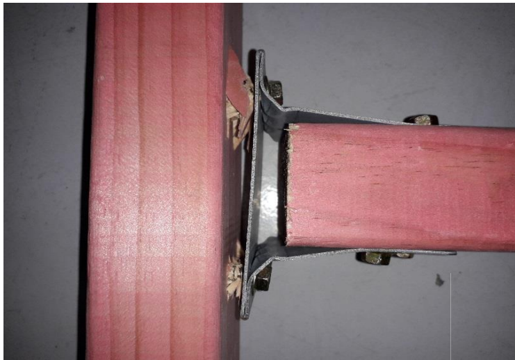
Figure 3 - Typical failure, screws pulling out of timber base.
