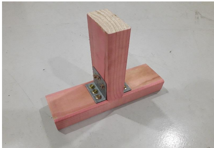
Figure 1 - JG2 bracket assembly as supplied
